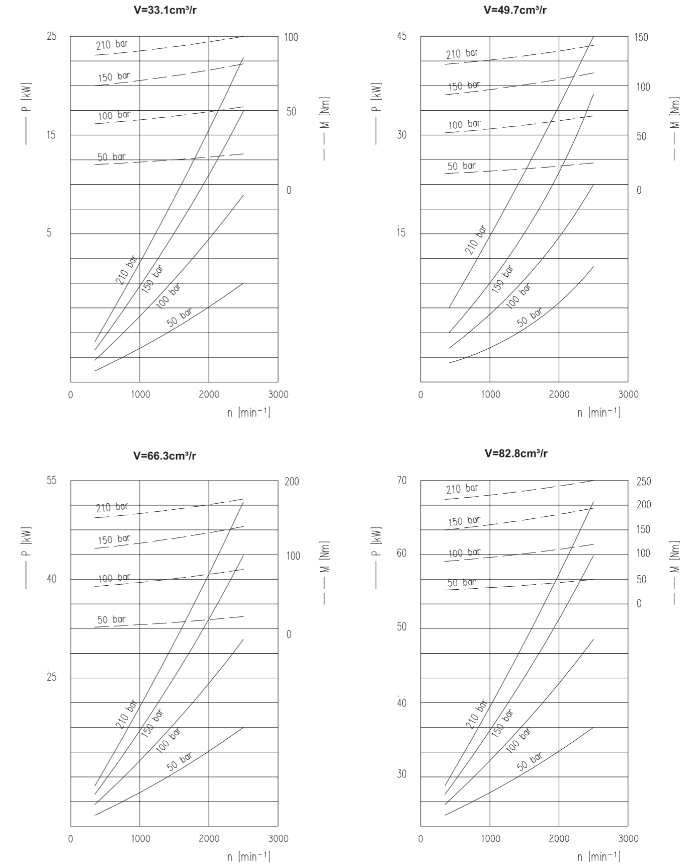
4系列功率性能曲线表/Group 4 Power Performance Curve Table
