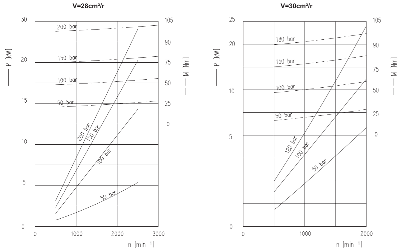
2系列功率性能曲线表/Group 2 Power Performance Curve Table
